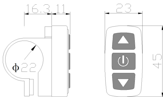
按钮盒外形尺寸
